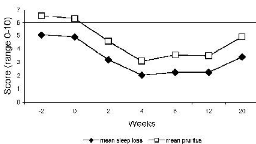
Figure 3: Symptoms score
